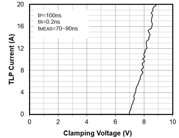
TLP Measurement
